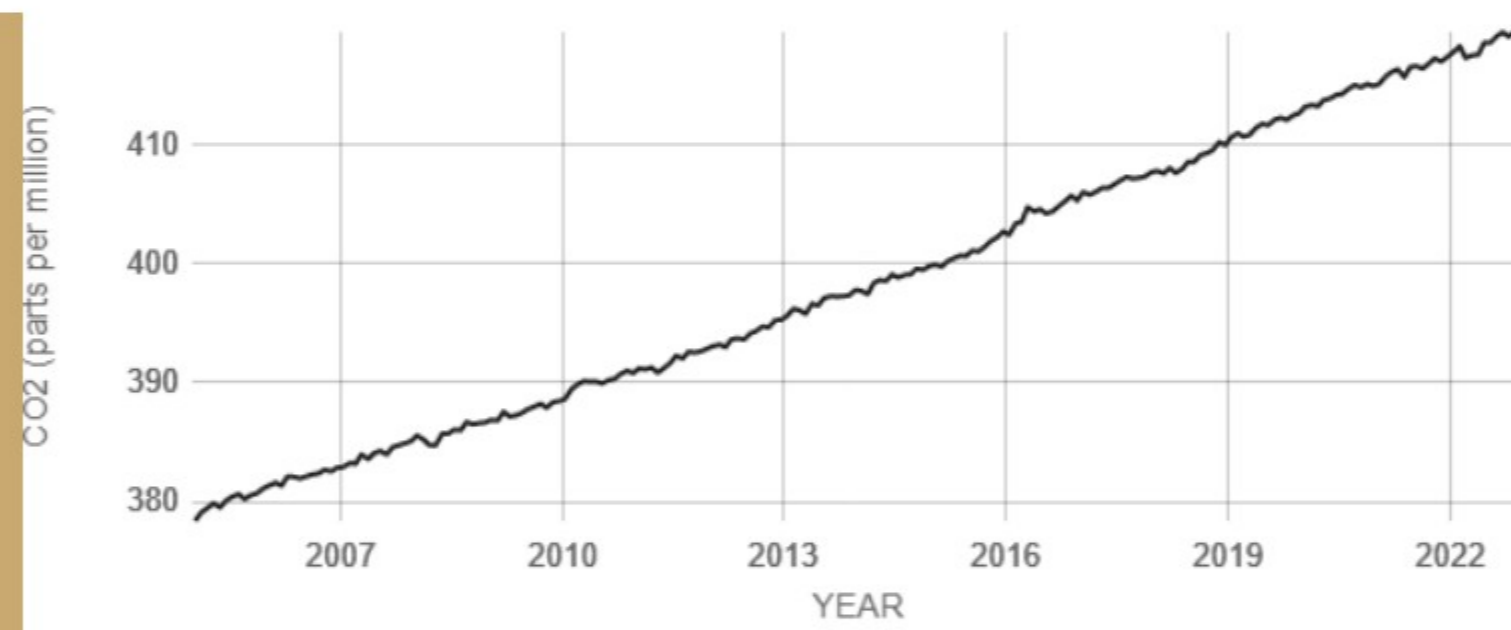
Source: climate.nasa.gov
