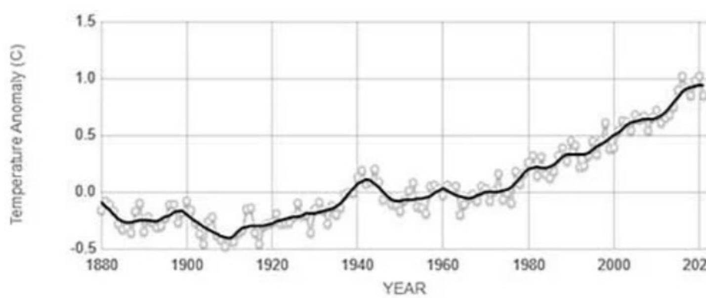
Source: climate.nasa.gov
